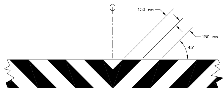
MARKING PLAN
