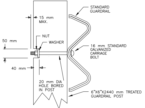
GUARDRAIL ATTACHMENT DETAIL
