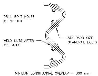
SPLICE DETAIL
